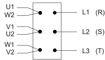
Panel connection
