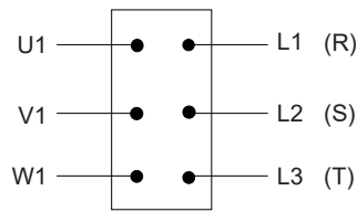
Panel connection
